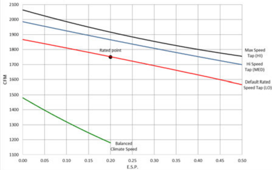
W60A Indoor Airflow Performance - Wet Coil
