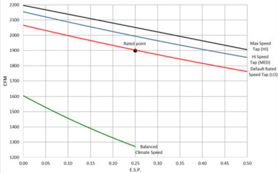
W72A Indoor Airflow Performance - Wet Coil
