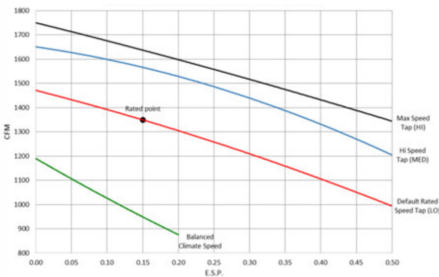
W48A Indoor Airflow Performance - Wet Coil
