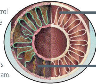
PROTECTED COPPER TUBING IN AN AIR COMPRESSOR UNPROTECTED COPPER TUBING IN AN AIR COMPRESSOR
